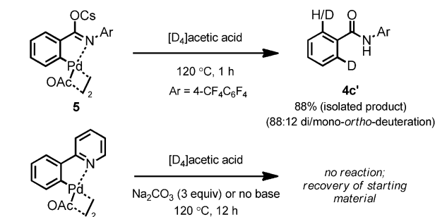
Scheme 4. ortho -Deuteration with palladacycles.
