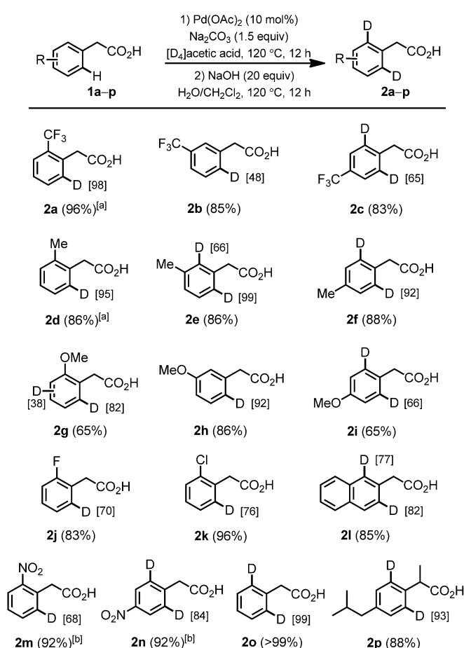
Scheme 2. Palladium-catalyzed ortho -deuteration of phenylacetic acids. Conditions for ortho -deuteration (in a 50 mL sealed tube):
